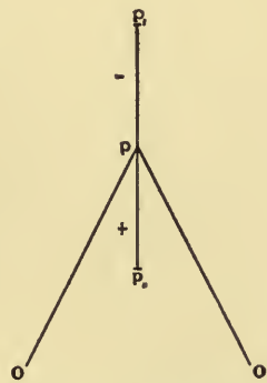
FIG. 208.—Illustration of relative accommodation.
